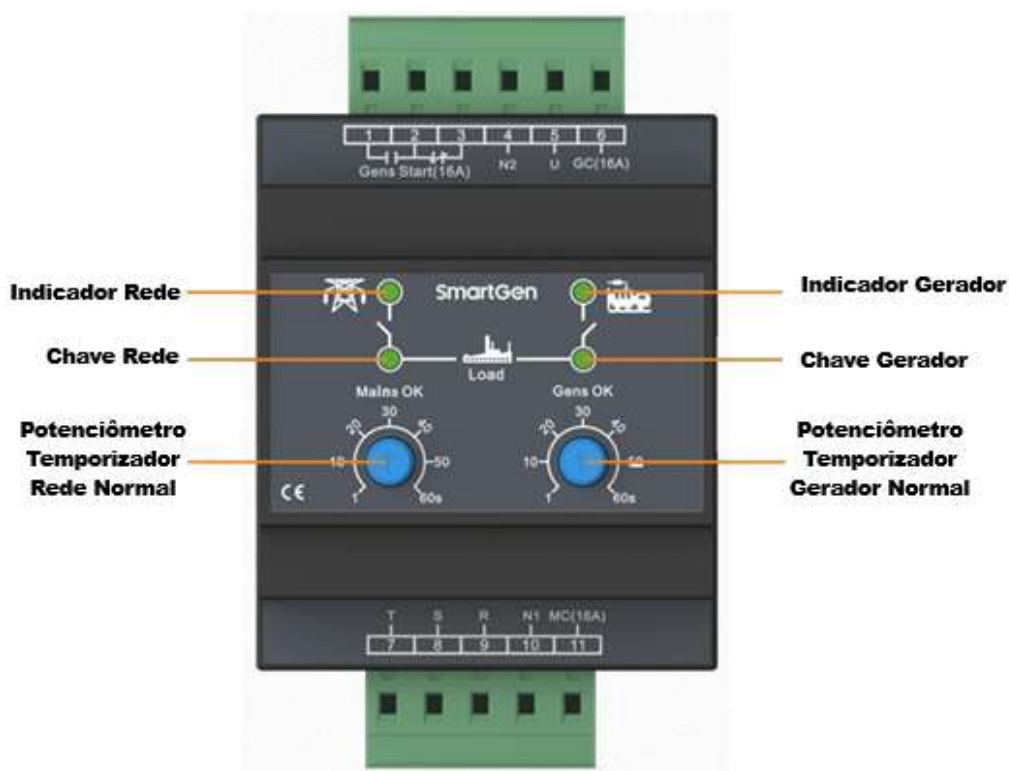
Figura 1 – Frontal HAT320
